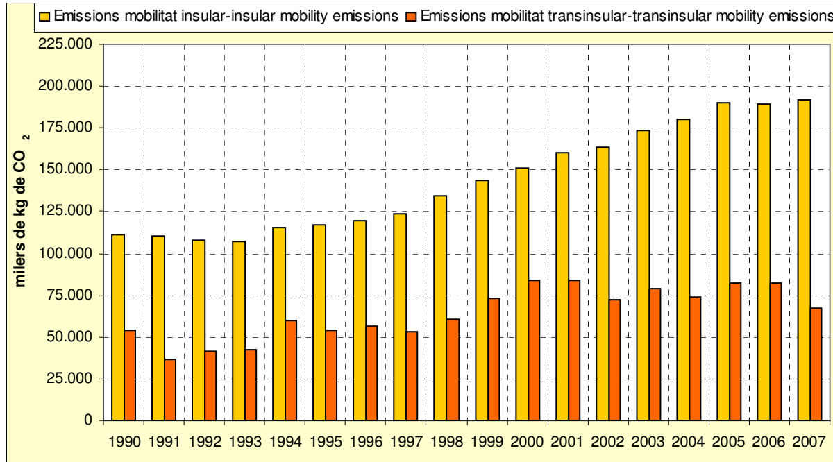
Graphic. 1. CO 2 emissions 1990-2007
